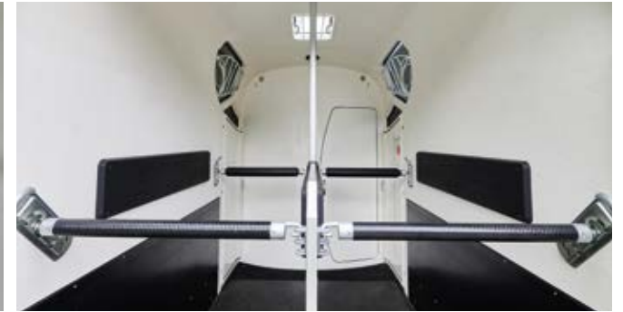
Strong dividing wall construction and high-quality materials with the solid, welded aluminium frame and the centre post dividing wall made of anodised aluminium.
